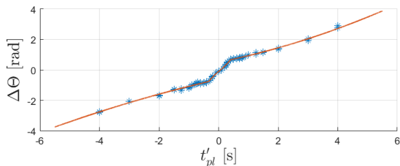
Fig. 5. Change in overall orientation per cycle for open-loop pause modulation over a base waveform defined by [T_1 \ T_2 \ A \ \phi_0] = [1.5 \ 1.5 \ 2 \ 0] . The signed pause-length t'_{pl} is defined as in (10). The data and best-fit function are shown.
