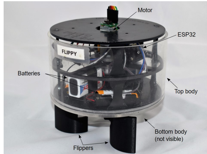
Fig. 1. The Modboat prototype, nicknamed Flippy. The bottom body is obscured beneath the top body [14].
