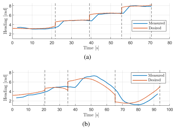
Fig. 9. Heading vs. time plots for the waypoint experiments in Fig. 8a. The pause controller is shown in (a), the frequency controller in (b). Vertical dotted lines show waypoints reached.
