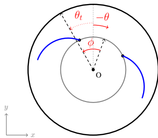
Fig. 2. A simplified top view of the Modboat. The bottom body is shown in gray with the flippers in blue, while the top body is black. The angles \theta and \theta_t are measured from the world frame y axis, while \phi is the relative angle between the two bodies.
