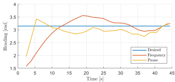
Fig. 7. Sample response of the two controllers to a step input of \approx \pi/2 ; control begins when the first heading measurement is obtained, at 1 cycle. The frequency controller lags significantly behind the pause controller.
