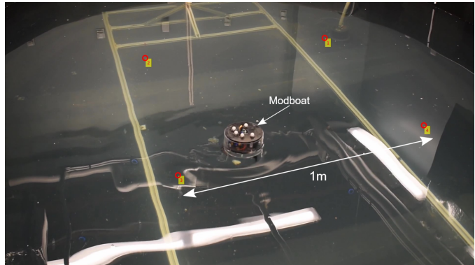
Fig. 6. A photo of the experimental setup, demonstrating the Modboat during a waypoint tracking experiment. The approximate locations of the waypoints are superimposed on the image.
